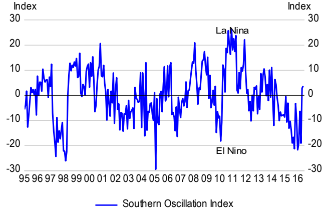
Source: www.longpaddock.qld.gov.au
