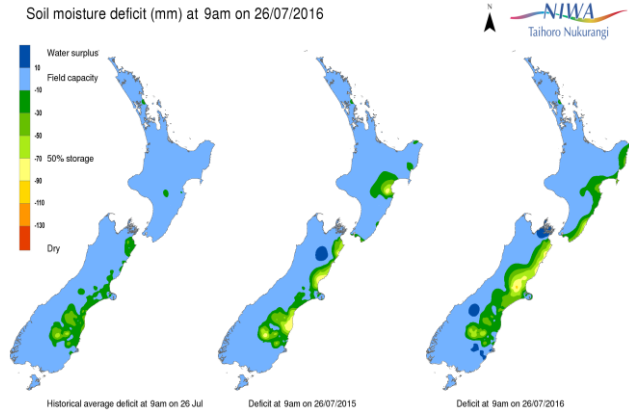
Source: NIWA
