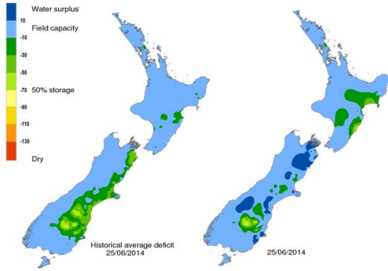
Source: NIWA
