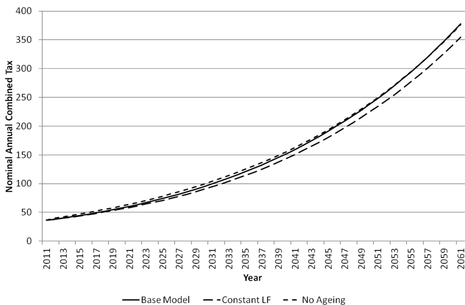
Figure 15: Effects of Ageing and Labour Force Participation: Male and Female and All Taxes Combined
