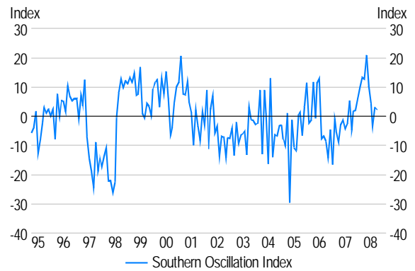
Source: www.longpaddock.qld.gov.au
