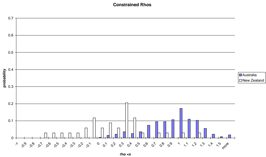
Figure 5: estimated distribution of \rho for New Zealand and Australia (equation 11)
